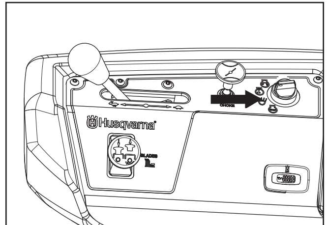
Ignition switch
