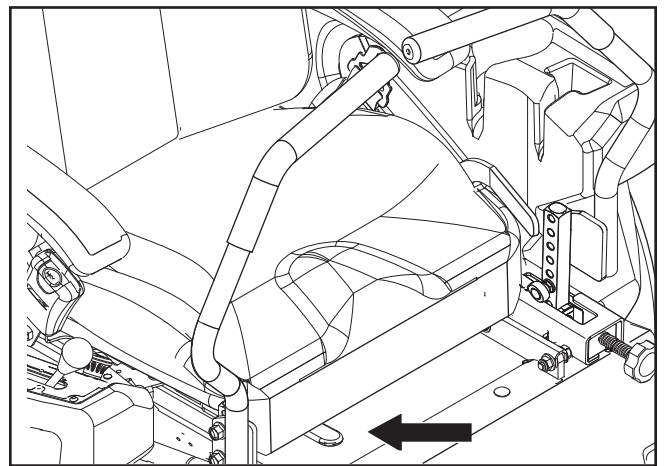
Seat adjustment
